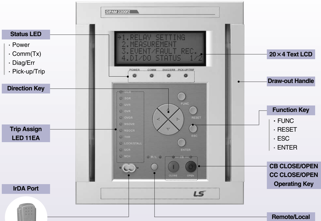
Front View
